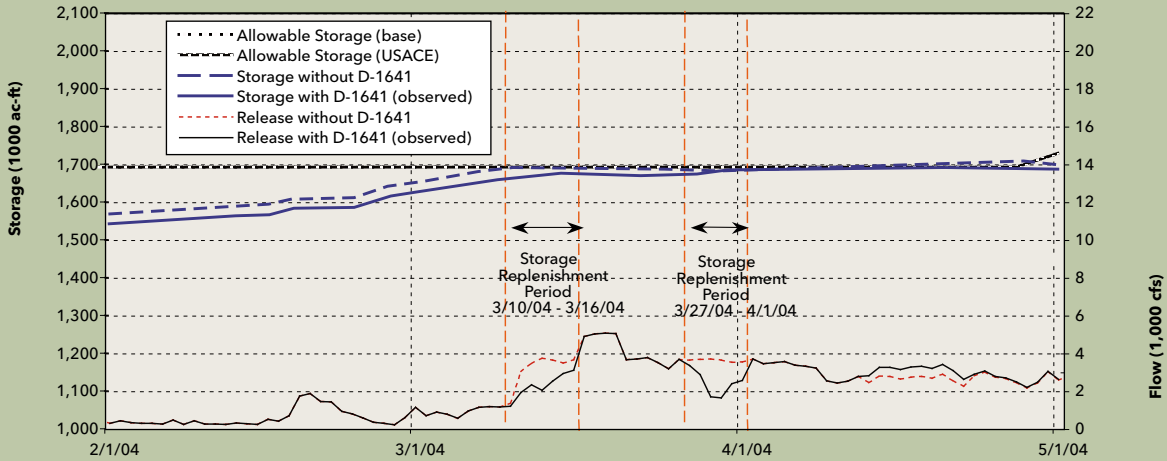
Appendix C, Figure 13 SWRCB D-1641 Reservoir Storage Replenishment in Don Pedro Reservoir (Tuolumne River) (Storage Replenishment Period: March 10 - 16, 2004 & March 27 - April 1, 2004)
