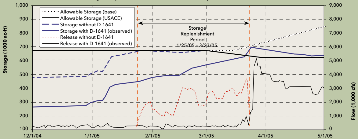
Appendix C, Figure 3 SWRCB D-1641 Reservoir Storage Replenishment in Lake McClure (Merced River) (Storage Replenishment Period: January 25 - March 23, 2005)
