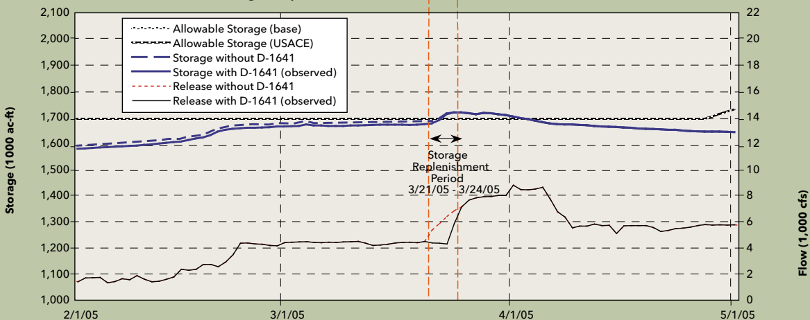
Appendix C, Figure 15 SWRCB D-1641 Reservoir Storage Replenishment in Don Pedro Reservoir (Tuolumne River) (Storage Replenishment Period: March 21 - 24, 2005)
