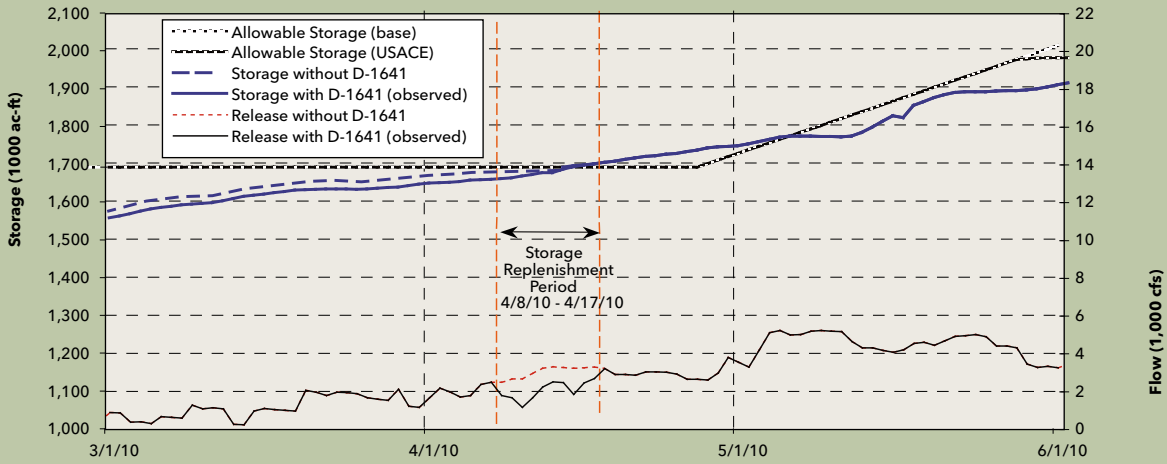
Appendix C, Figure 17 SWRCB D-1641 Reservoir Storage Replenishment in Don Pedro Reservoir (Tuolumne River) (Storage Replenishment Period: April 8 - 17, 2010)
