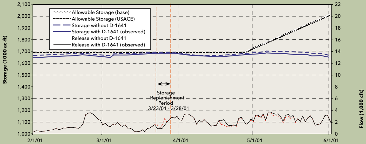
Appendix C, Figure 11 SWRCB D-1641 Reservoir Storage Replenishment in Don Pedro Reservoir (Tuolumne River) (Storage Replenishment Period: March 23 - 28, 2001)
