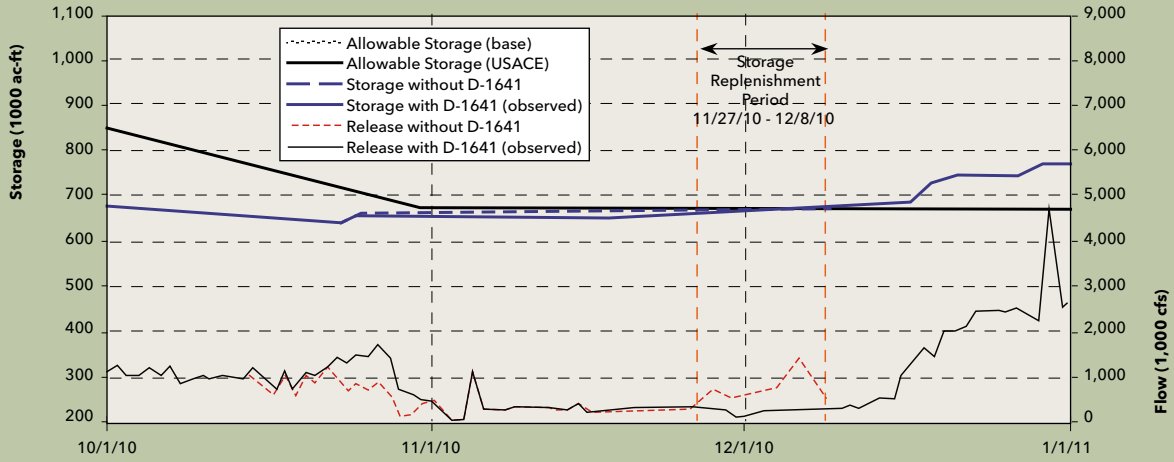
Appendix C, Figure 7 SWRCB D-1641 Reservoir Storage Replenishment in Lake McClure (Merced River) (Storage Replenishment Period: November 27 - December 8, 2010)
