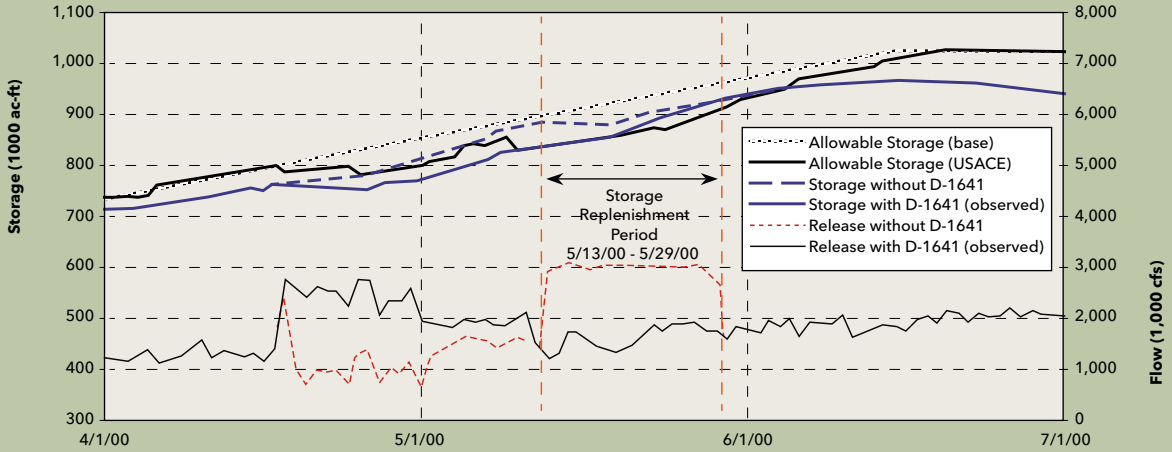
Appendix C, Figure 1 SWRCB D-1641 Reservoir Storage Replenishment in Lake McClure (Merced River) (Storage Replenishment Period: May 13 - 29, 2000)
