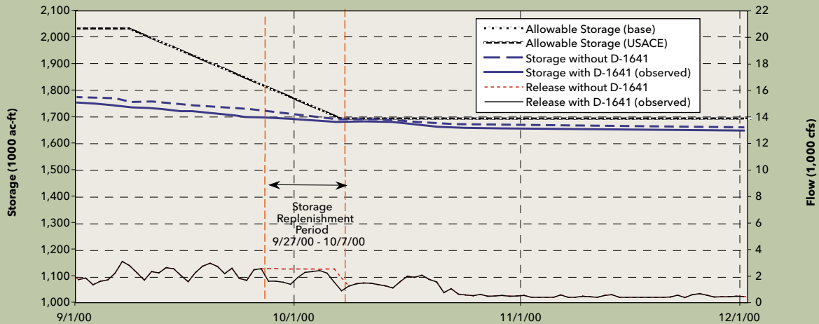
Appendix C, Figure 9 SWRCB D-1641 Reservoir Storage Replenishment in Don Pedro Reservoir (Tuolumne River) (Storage Replenishment Period: September 27 - October 7, 2000)
