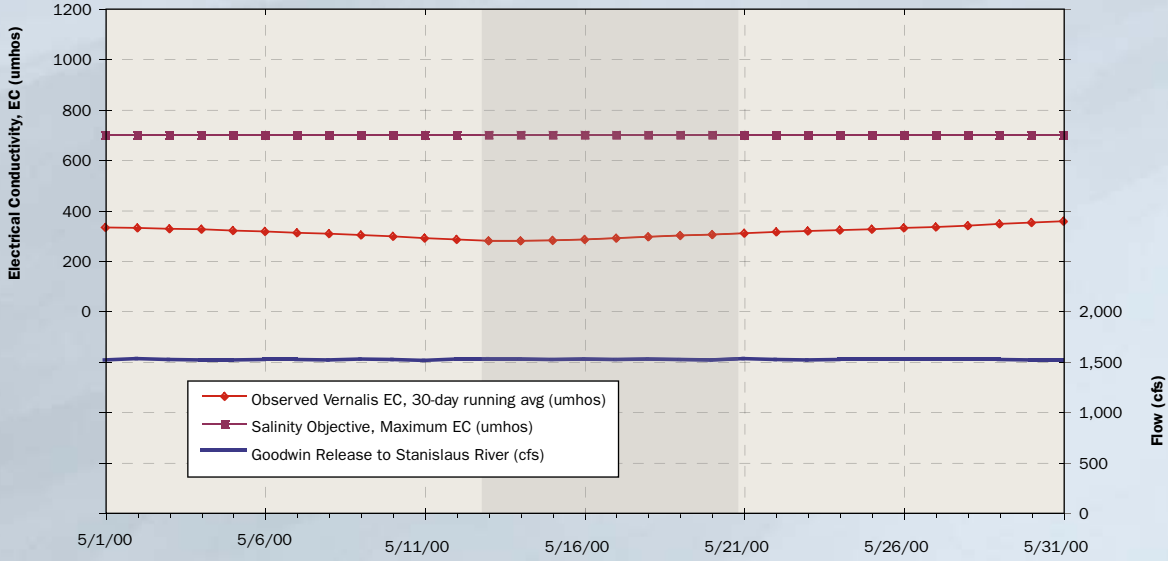
Appendix D, Figure 1 Impact of SWRCB D-1641 Storage and Flow Conditions on Vernalis Water Quality and Goodwin Dam Release to Stanislaus River, May 2000
