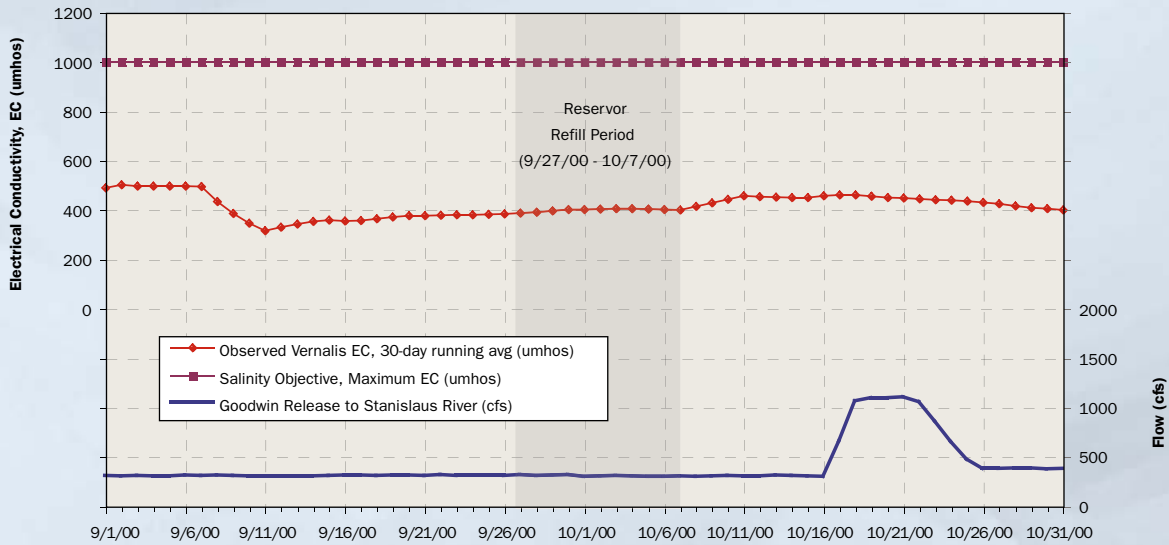
Appendix D, Figure 2 Impact of SWRCB D-1641 Storage and Flow Conditions on Vernalis Water Quality and Goodwin Dam Release to Stanislaus River, September - October 2000 (Reservoir Refill Period: September 27 – October 7, 2000)
