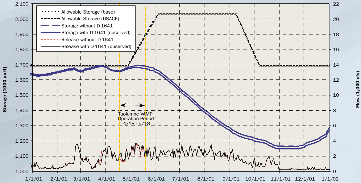
Appendix C, Figure 3 Impact of SWRCB D-1641 Storage and Flow Conditions on Don Pedro Reservoir Storage and Release (Tuolumne River) for 2001. (Refill period: March 23 – 28, 2001)
