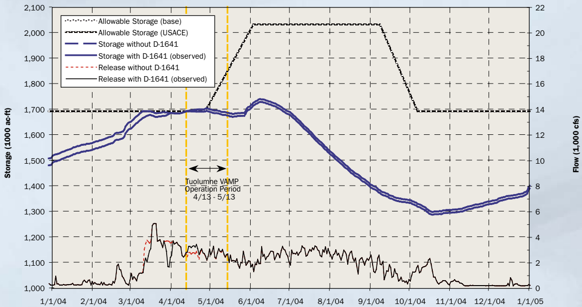
Appendix C, Figure 4 Impact of SWRCB D-1641 Storage and Flow Conditions on Don Pedro Reservoir Storage and Release (Tuolumne River) for 2004. (Refill period: March 10 – 16, 2004 and March 27 – April 1, 2004)
